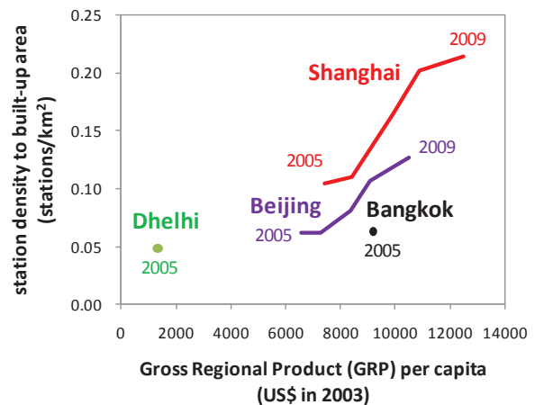
Fig 3 Changes in railway development according to economic growth (Built-up area is fixed to be the level of 2005.)
