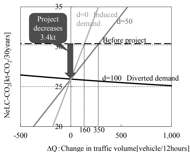
Figure 11. Sensitivity analysis with change in traffic demand for crossing A
